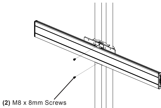
Single Mounting Bracket
