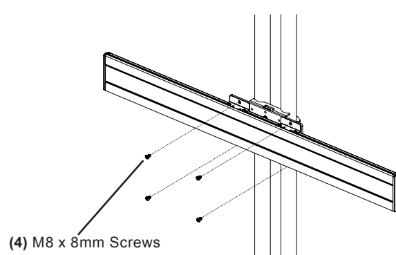
Double Mounting Bracket
