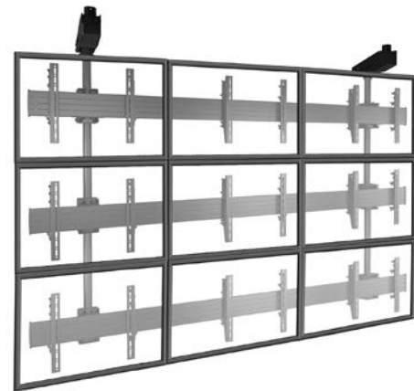
LCM3x3U 3 x 3 Video Wall Solution
