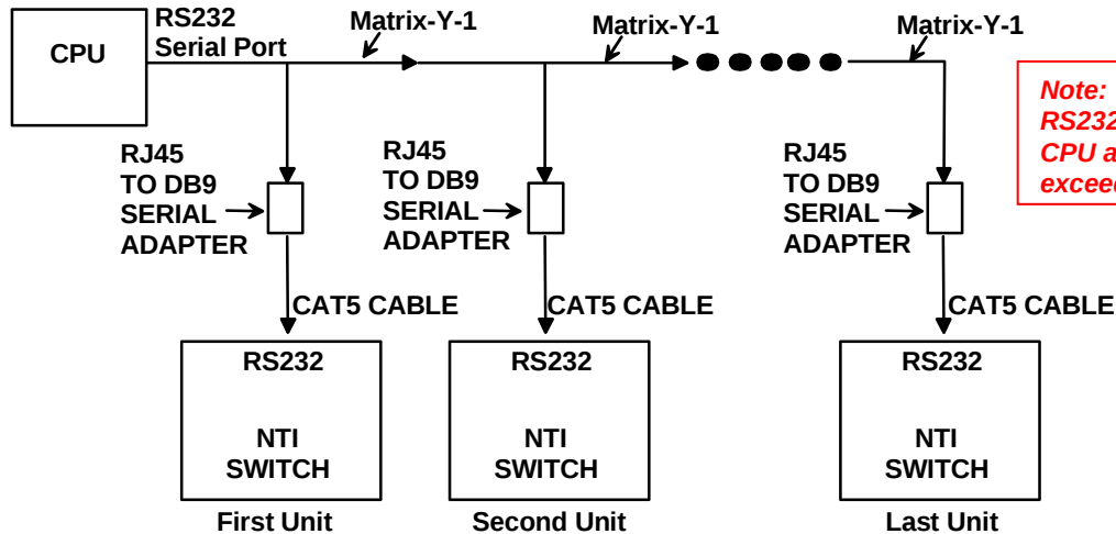
Figure 33- RS232 connection with Matrix-Y-1 cable
