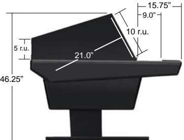
V Series profile with V1005 rack module.
